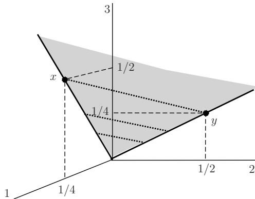
The cone generated by x and y consists of similar points. Each dotted line consists of points which on top of being similar have also the same probability.
